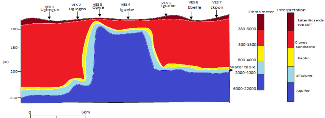
Fig. 7. Geo-electrical resistivity section of the study area
