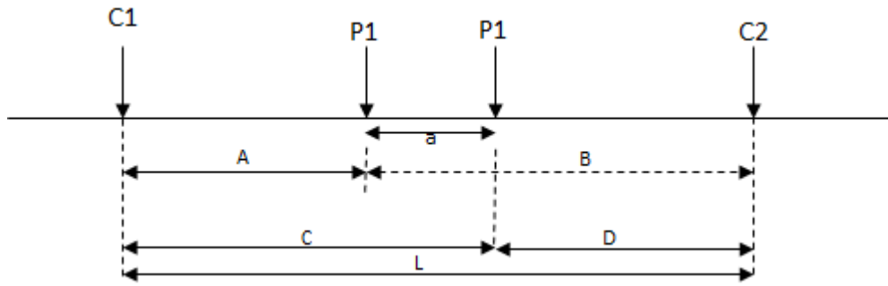
Fig. 4. Schlumberger array After Lowrie, [13]
