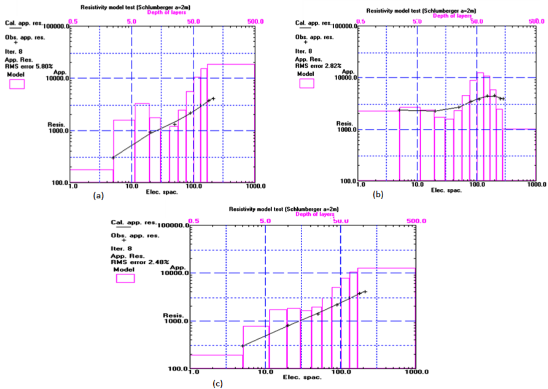
Fig. 6. (a) Inverted model layer for VES 5 taken at Iguebe south (2) Inverted model layer for VES 6 taken at Ebelle (c) Inverted model layer for VES 7 taken at Ekpon in Edo State
