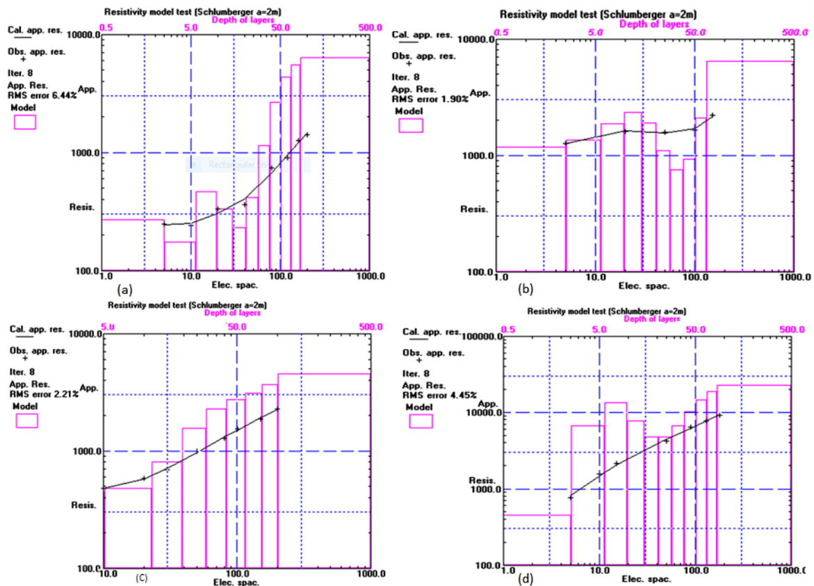
Fig. 5. (a) Inverted model layer for VES 1 taken at Ugbegun (b) Inverted model layer for VES 2 taken at Ugiogba (c) Inverted model layer for VES 3 taken at Ogwa (d) Inverted model layer for VES 4 taken at Iguebe north in Edo State
