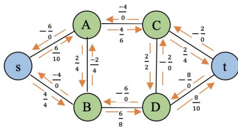
Fig. 2. Illustration of flow and capacity in a flow network
