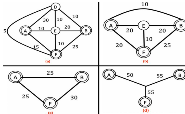
Fig. 17. Transformation procedure for the flow network in Fig. 16
