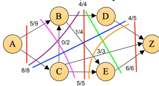
Fig. 10. A 9-branch flow network with all 8 possible cuts for Example 4
