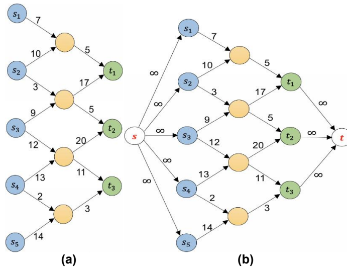
Fig. 1. Conversion of a multiple-source, multiple-sink maximum-flow problem for the telecommunication wireless network into a problem with a single source and a single sink. The figure (a) above shows how to transform a multiple-source, multiple-sink maximum-solution problem for the telecommunication wireless network into a single-source and a single-sink problem. It has a five-source S = \{s_1, s_2, s_3, s_4, s_5\} flow network with three sinks T = \{t_1, t_2, t_3\} . Diagram (b) shows the corresponding network flow for a single-source and a single-sink. The significant changes made in going from (a) to (b) include the addition of a super-source s and an edge with an unlimited (or sufficient) capacity from s to each of the multiple sources, the addition of a super-sink t and an edge with an unlimited (or sufficient) capacity from each of the multiple sinks to t
