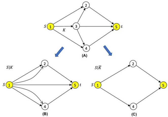
Fig. 19. Decomposition technique for evaluating complex systems' reliability
