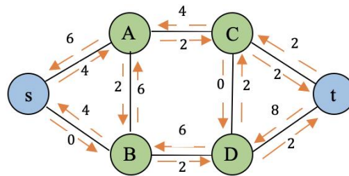
Fig. 3. The flow network in Fig. 2 redrawn to show the residual capacities
