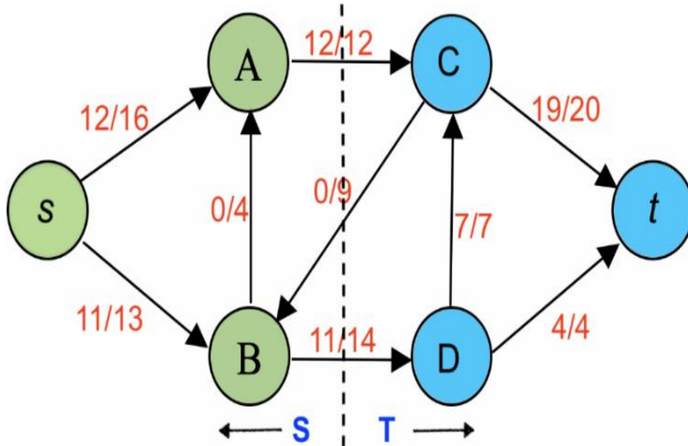
Fig. 5. A cut (S, T) for a specific flow network, where S = \{s, A, B\} and T = \{C, D, t\} . The vertices in S are green, and the vertices in T are blue. The net flow across (S, T) is f(S, T) = 23 , and the capacity is c(S, T) = 26
