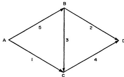
Fig. 6. A simple capacitated (flow) network
