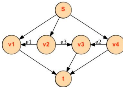
Fig. 4. A flow network for which the Ford-Fulkerson does not terminate
