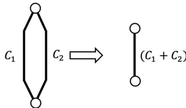
Fig. 12. Network simplification of branches in parallel
