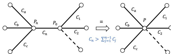
Fig. 13. Network simplification of branches for Rule 3
