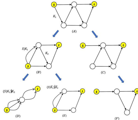
Fig. 20. Decomposition-based technique for determining a topologically complex network's reliability on sequential selection of two keystone components
