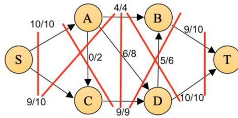
Fig. 9. A 9-branch flow network with all 7 possible cuts for Example 3 with a maximum flow value of 19 across each of them, with only one of them saturated
