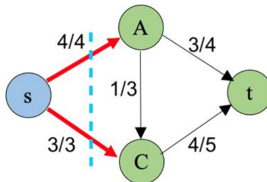
Fig. 8. A network with a value of flow that equals the capacity of an s - t cut
