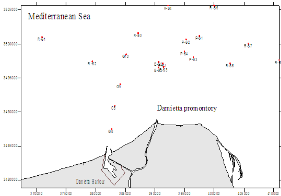
Fig 3. Study area showing locations of surficial sediment samples of the continental shelf between the Damietta Harbor and Damietta promontory R-S = disposal site reference samples, E-S = existing disposal site, P-S = proposed disposal site, G8-G10 = grab sample and C6 = core position.
