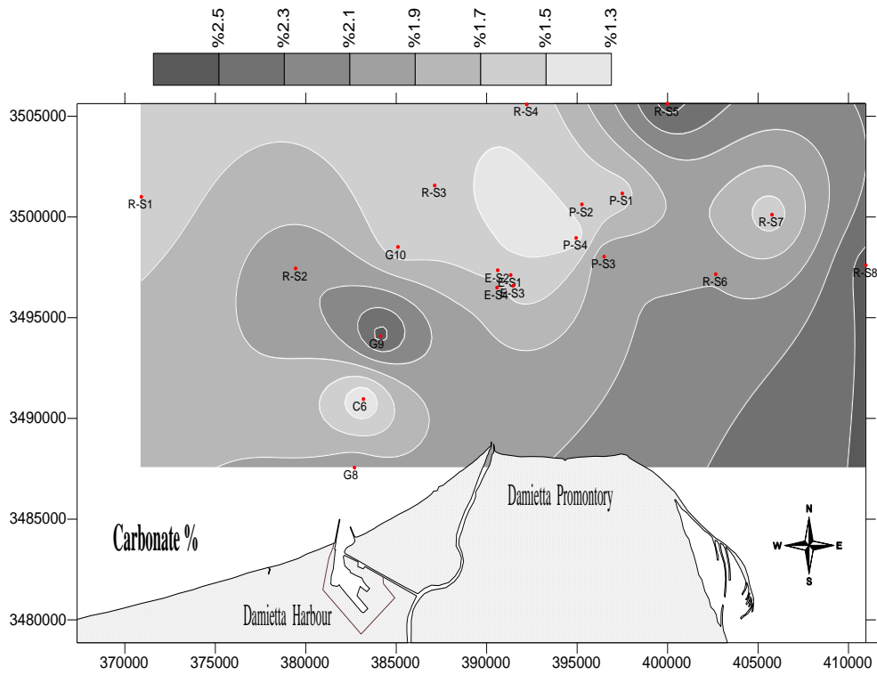
Fig. 14. Offshore geographical distribution of carbonate %
