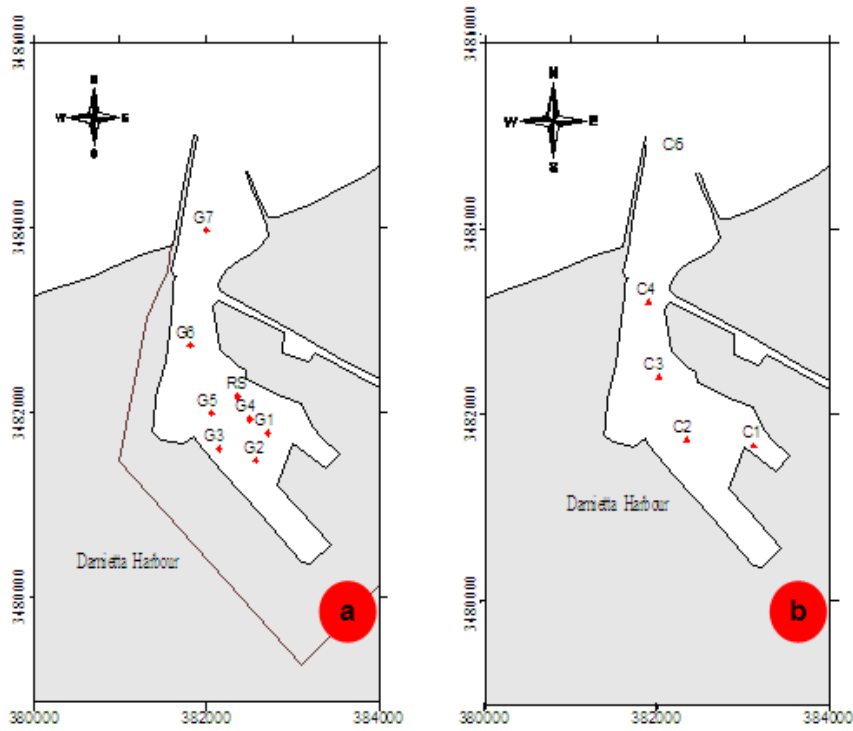
Fig. 2. Study area showing locations of the followings: a) Grab sediment samples (G1 to G7 and RS) in the Damietta Harbor basin, and b) Sediment cores (Core 1 to Core 6)
