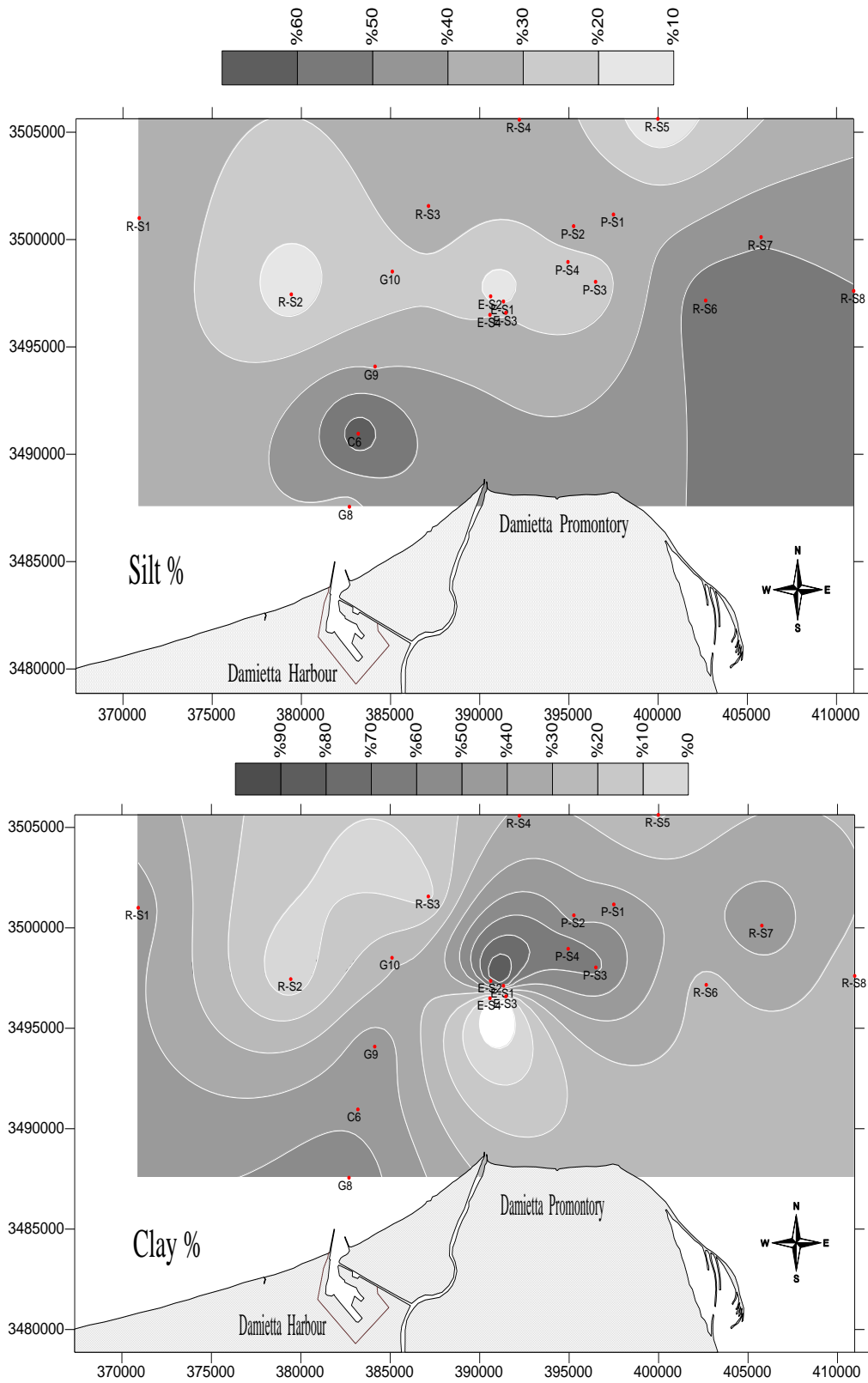
Fig. 8. Offshore geographical distribution of a) sand%, b) silt% and c) clay% of Damietta
