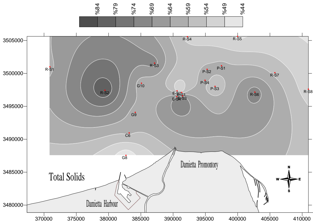
Fig. 12. Offshore geographical distribution of total solids %
