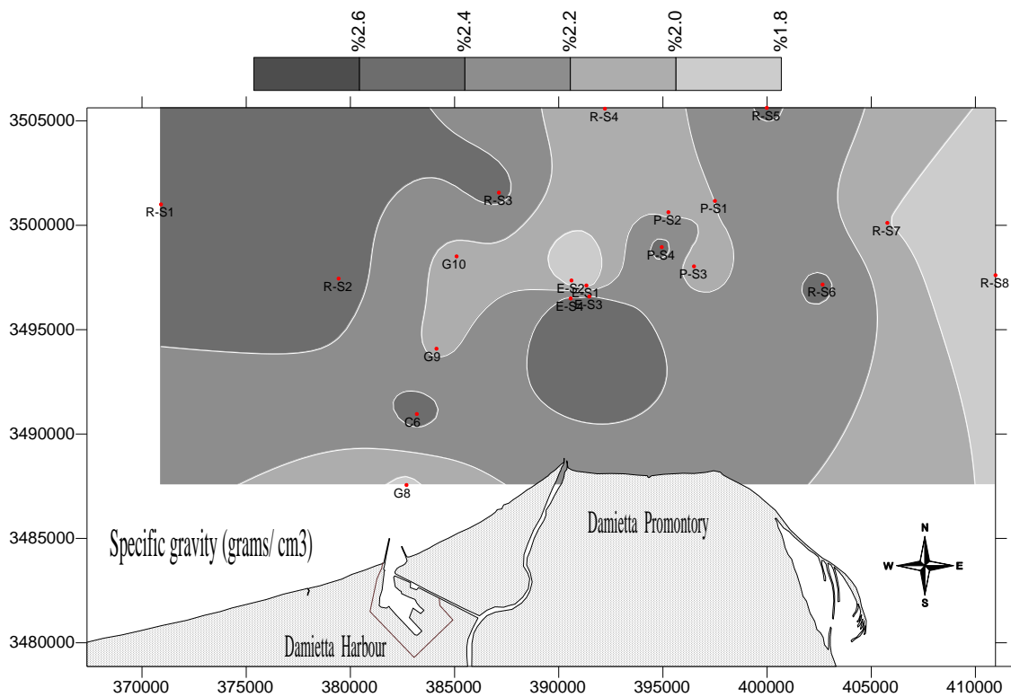
Fig. 18. Offshore geographical distribution of specific gravity (gram/cm 3 )
