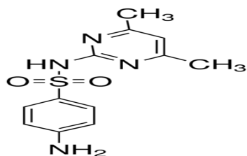
Fig. 1. Molecular structure of Sulfamethazine (SMT)
