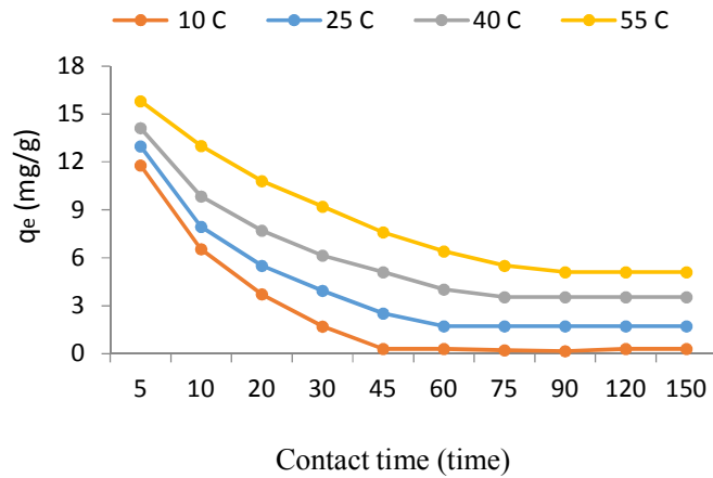
Fig. 3. Effect of contact time and temperature on the removal of SMT by TTRH (concentration: 50 mg/L; dose: 2.5 g/L; shaking speed: 180 rpm; pH: 7)
