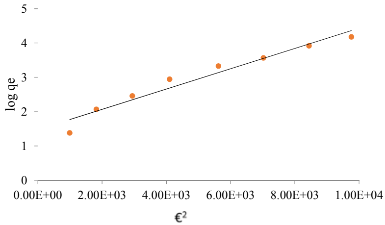
Fig. 2C. Dubinin–Radushkevich isotherm models for the adsorption of SMT adsorption onto TTRH
