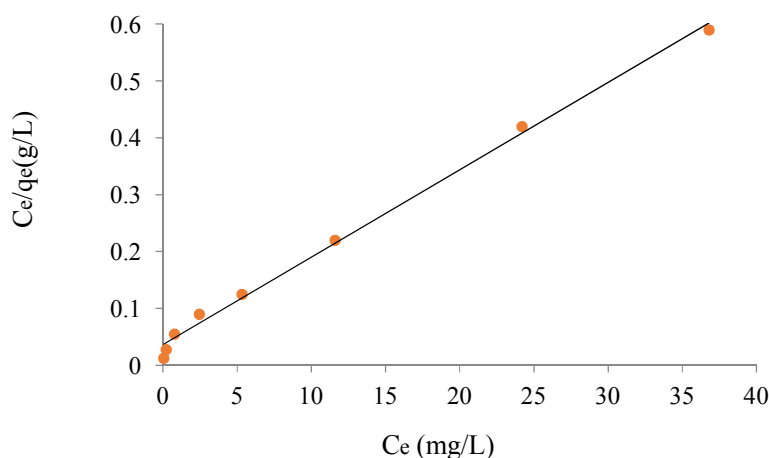
Fig. 2a. Langmuir isotherm models for the adsorption of SMT adsorption onto TTRH
