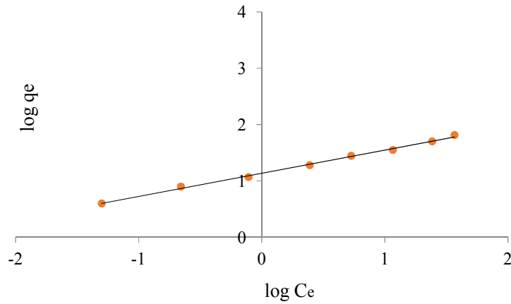
Fig. 2b. Freundlich isotherm models for the adsorption of SMT adsorption onto TTRH
