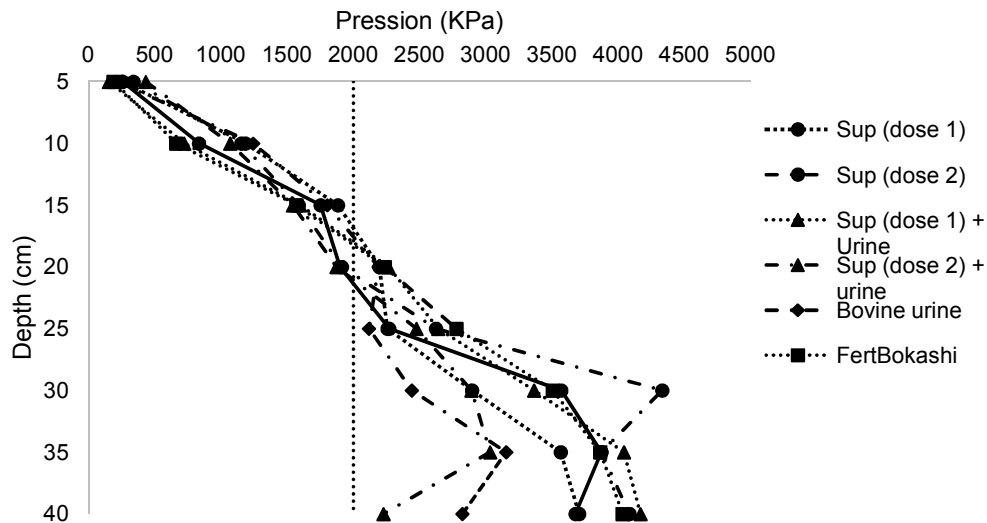
Fig. 1. Effect of the treatments in the soil penetration resistance (KPa), in the depth of 5 to 40 centimeters
