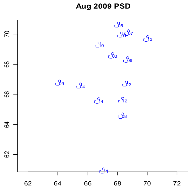
Fig. 4b. Metric MDS for August PSD
