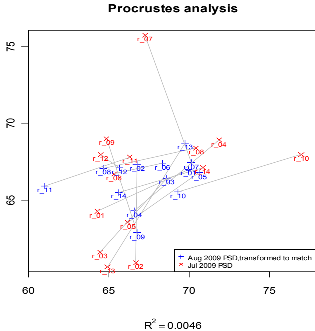
Fig. 5b. Procrustes Analysis for PSD (August matched to July)
