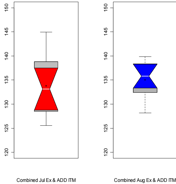
Fig. 3. Combined box plot for Ex-ITM and Ex-ADD
