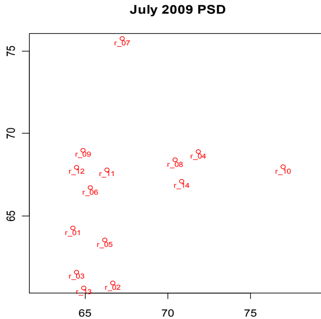
Fig. 4a. Metric MDS for July PSD
