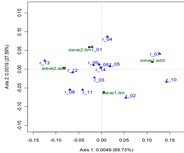
Fig. 7. Correspondence analysis plot August PSD data set (symmetric map)
