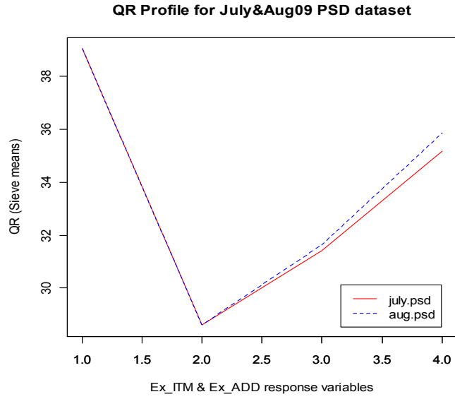
Fig. 1. Profile plot for PSD data set
