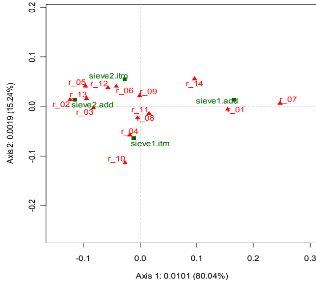
Fig. 6. Correspondence analysis plot for July PSD data set (symmetric map)
