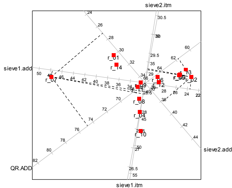
Fig. 8. PCA biplot for July PSD data set (Quality of Display = 88.65%)
