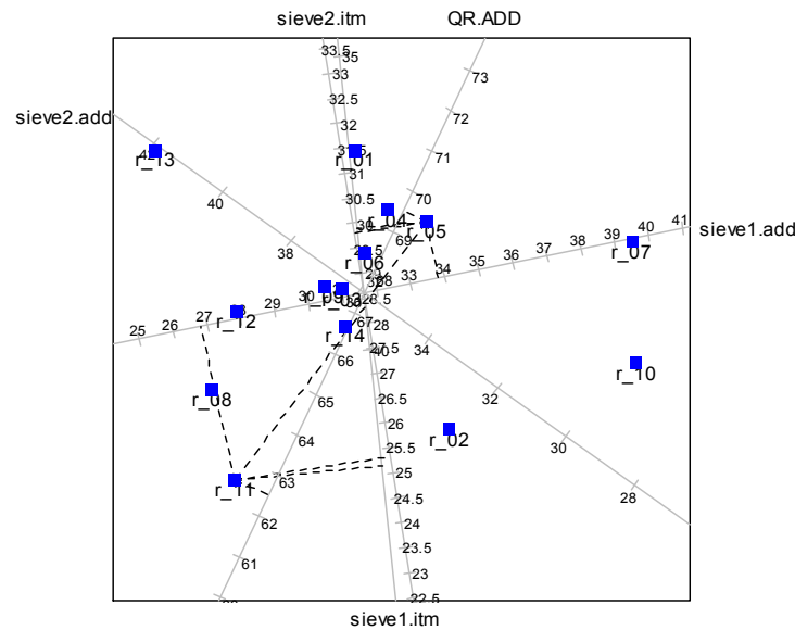
Fig. 9. PCA biplot for August PSD data set (Quality of Display = 85.65%)
