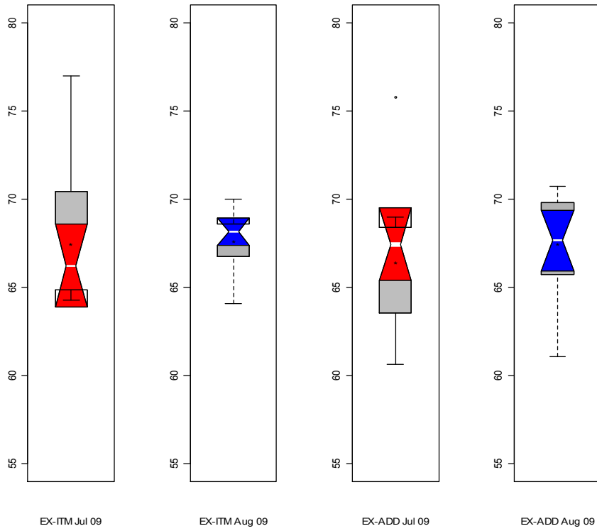
Fig. 2. Box plots for July and August Ex-ITM and Ex-ADD
