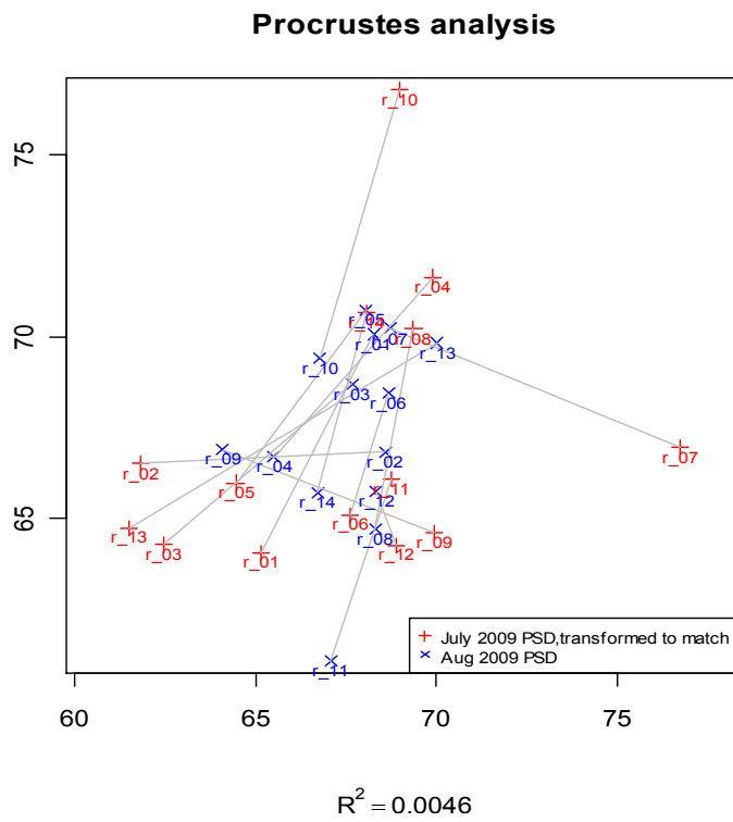
Fig. 5a. Procrustes analysis for PSD (July matched to August)
